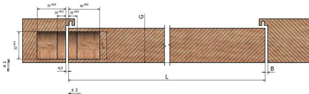
Dimensions of socket
